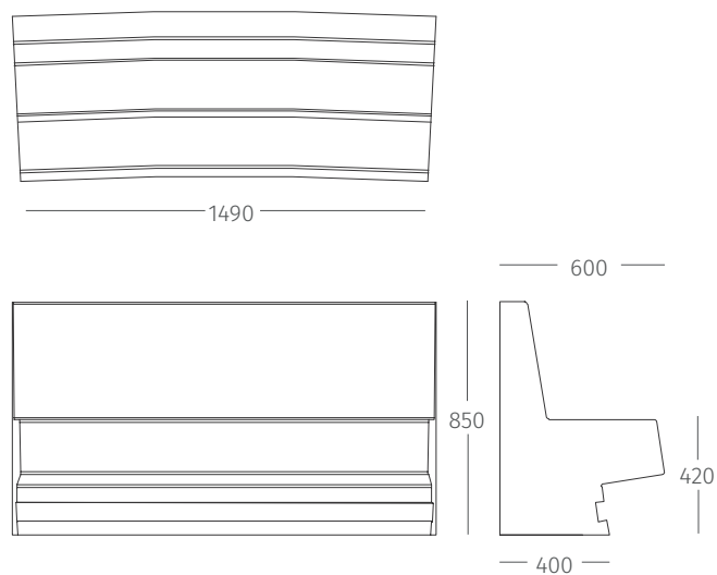
Bequer konkav, r = 14,7\text{ m}
