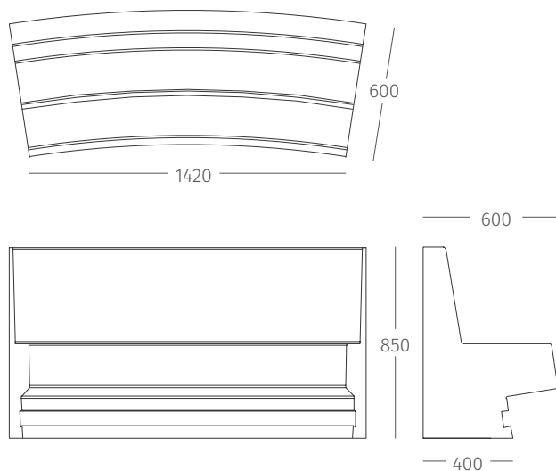
Bequer konkav, r = 4,7\text{ m}
